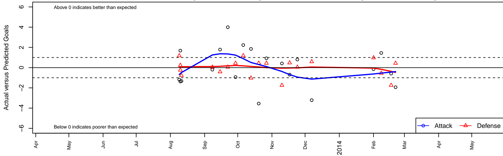
Sparta B96 Dots are actual minus expected GF (blue circles) and GA (red triangles). Blue line is smoothed change in attack strength. Red is smoothed change in defense strength.
